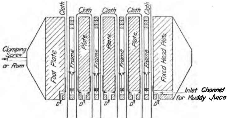
FIG. 20.—FLOW OF JUICE DURING FILTRATION
